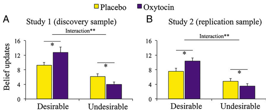
Fig. 1. Distinct OT effects on belief updates upon desirable and undesirable feedback in studies 1 (A) and 2 (B). IN-OT enhanced belief updating upon desirable feedback, but decreased belief updating upon undesirable feedback. * P < 0.05 ; ** P < 0.01 .
